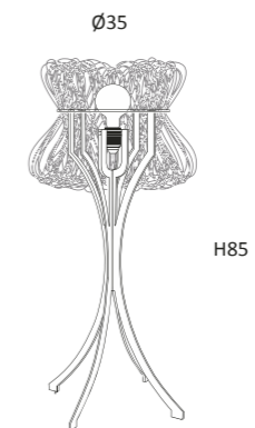
CLOCHE Table 35 1 x 8W LED E26/E27 Material: 2 mm wire rope, corddimmer integrated
